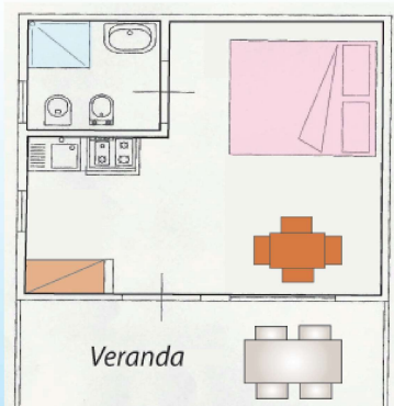
Bungalow Monolocale - mq.16
